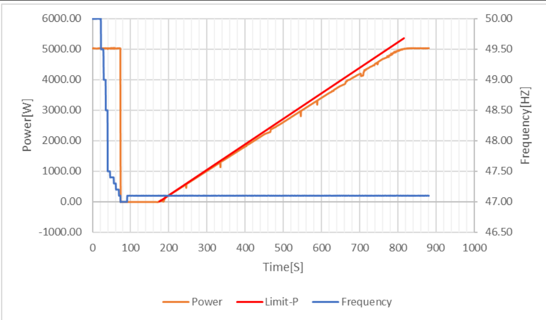
Recovery after under Frequency, Graph
