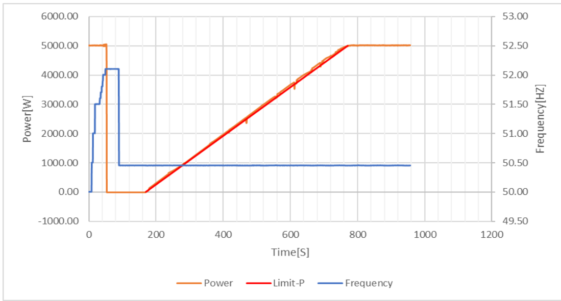
Recovery after Over Frequency, Graph
